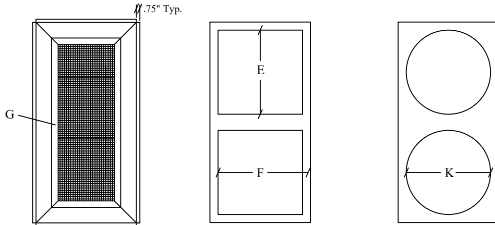
TYPICAL HARD DUCT CONNECTION OR TYPICAL FLEX DUCT CONNECTION
